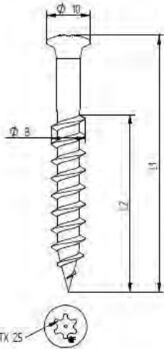
VRF Eurofast GBS 8,0 x L
